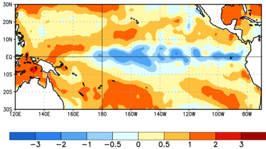
Figure 1. Average sea surface temperature (SST) anomalies (°C) for the week centered on 5 October 2016. Anomalies are computed with respect to the 1981-2010 base period weekly means.
