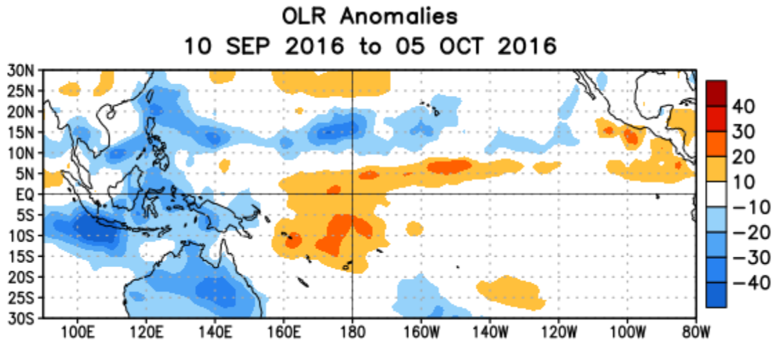
Figure 5. Average outgoing longwave radiation (OLR) anomalies ( W/m^2 ) for the period 10 September – 5 October 2016. OLR anomalies are computed as departures from the 1981-2010 base period pentad means.
