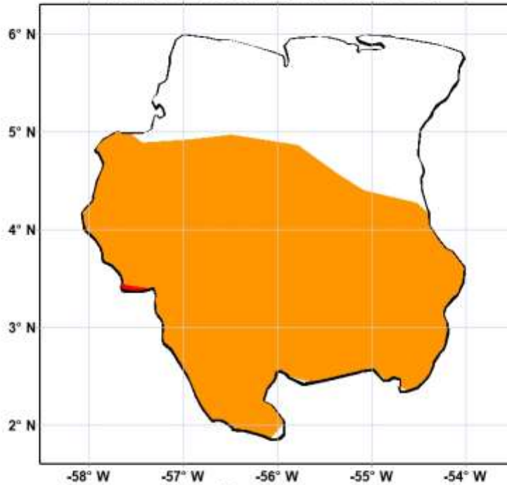
Week-1 Suriname Heat Hazard Outlooks Valid: 29 Jan - 04 Feb 2025
