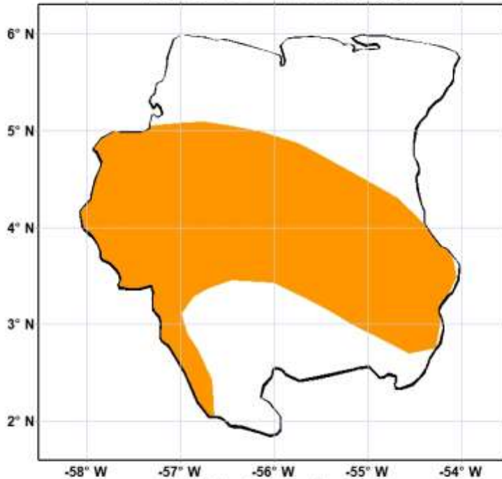
Week-2 Suriname Heat Hazard Outlooks Valid: 05 - 11 Feb 2025
