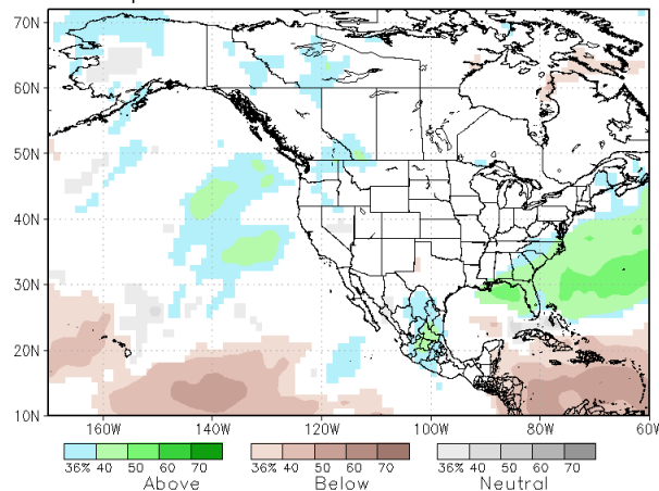
NMME prob fcast Prate IC=201811 for lead 1 2018 DJF
