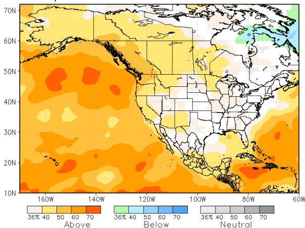
NMME prob fcast TMP2m IC=201811 for lead 1 2018 DJF
