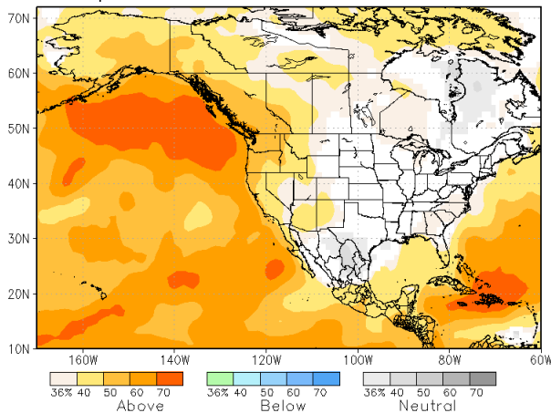
NMME prob fcst TMP2m IC=201812 for lead 1 2019 JFM
