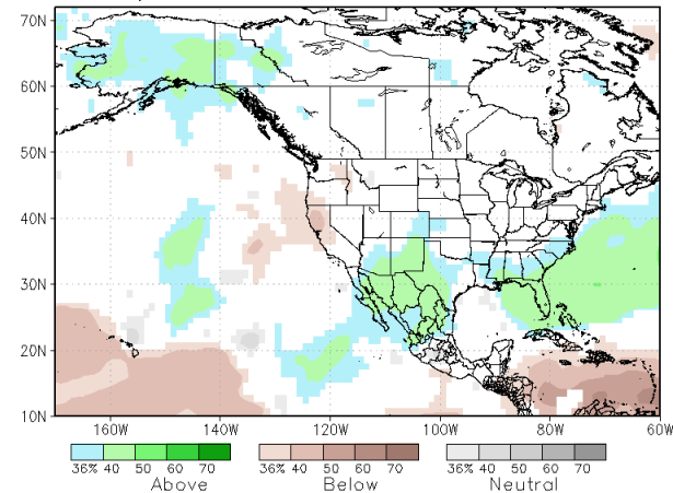
NMME prob fcst Prate IC=201812 for lead 1 2019 JFM
