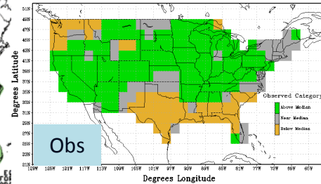
Categorical Precipitation Observations Valid: Jan-Feb-Mar 2019
