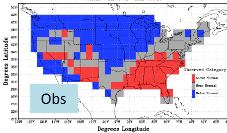
Categorical Temperature Observations Valid: Jan-Feb-Mar 2019
