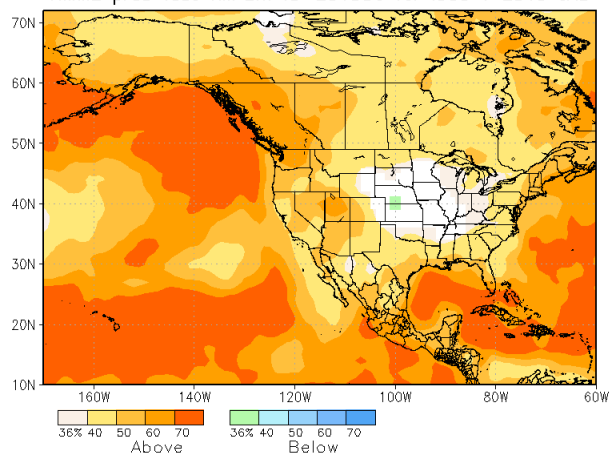
NMME prob fcst TMP2m IC=201906 for lead 1 2019 JAS
