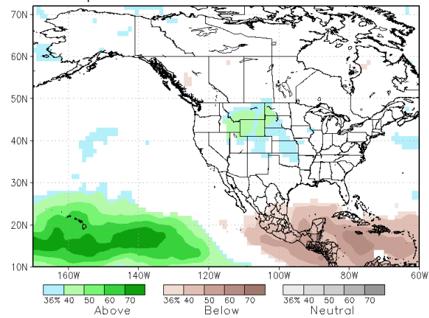
NMME prob fcst Prate IC=201906 for lead 1 2019 JAS
