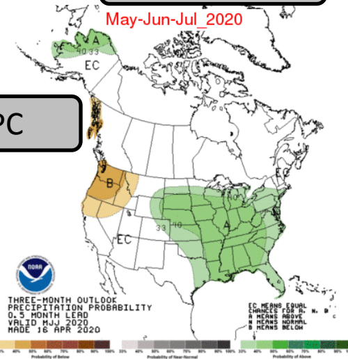
NMME prob fcst Prate IC=202004 for lead 1 2020 MJJ
