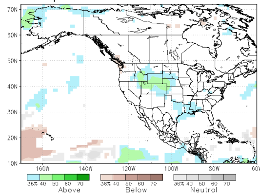
NMME prob fcst Prate IC=202004 for lead 1 2020 MJJ
