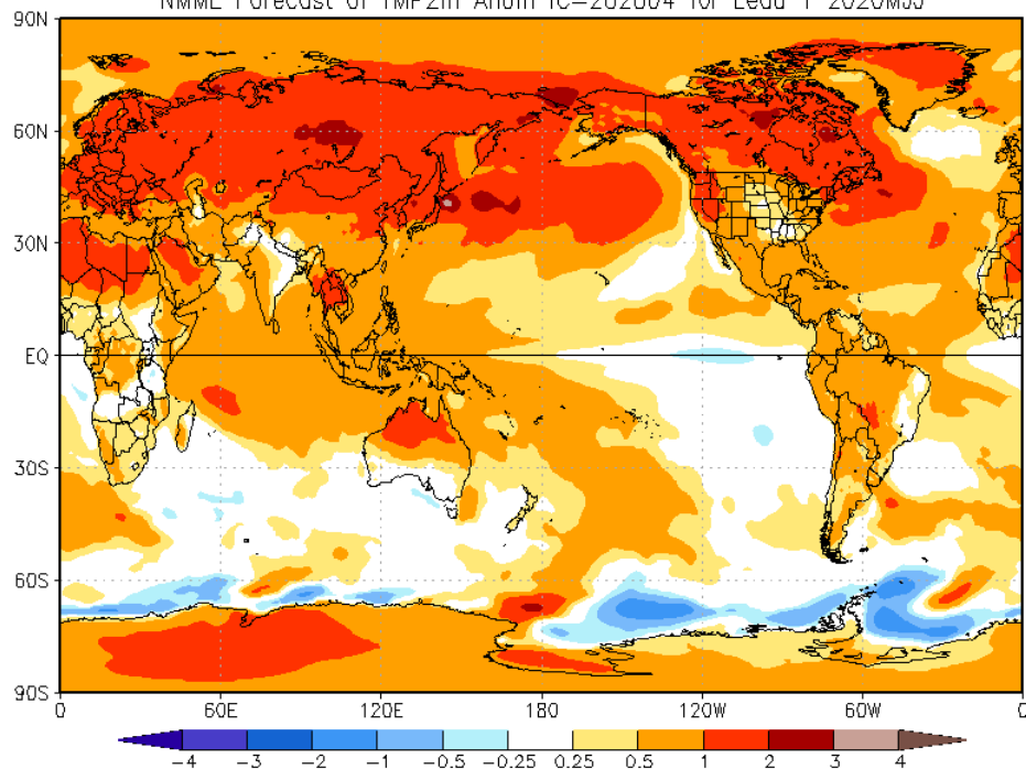
NMME Forecast of TMP2m Anom IC=202004 for Lead 1 2020MJJ
