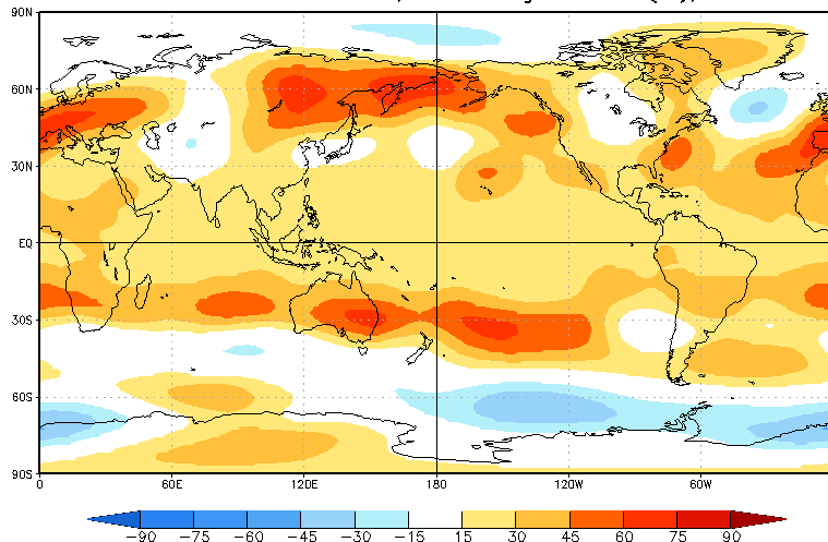
CA HGT200 Prd for MJJ2020, ICs through Jul2020(m), Lead -3
