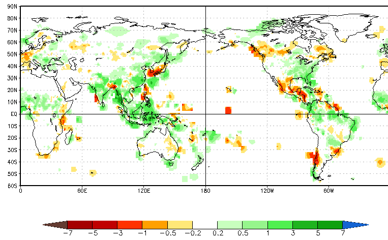
CA Prec Prd for MJJ2020, ICs through Jul2020(mm/day), Lead -3
