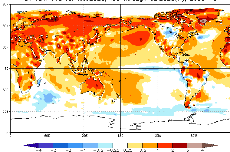
CA T2m Prd for MJJ2020, ICs through Jul2020(K), Lead -3
