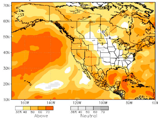
NMME prob fcst TMP2m IC=202004 for lead 1 2020 MJJ
