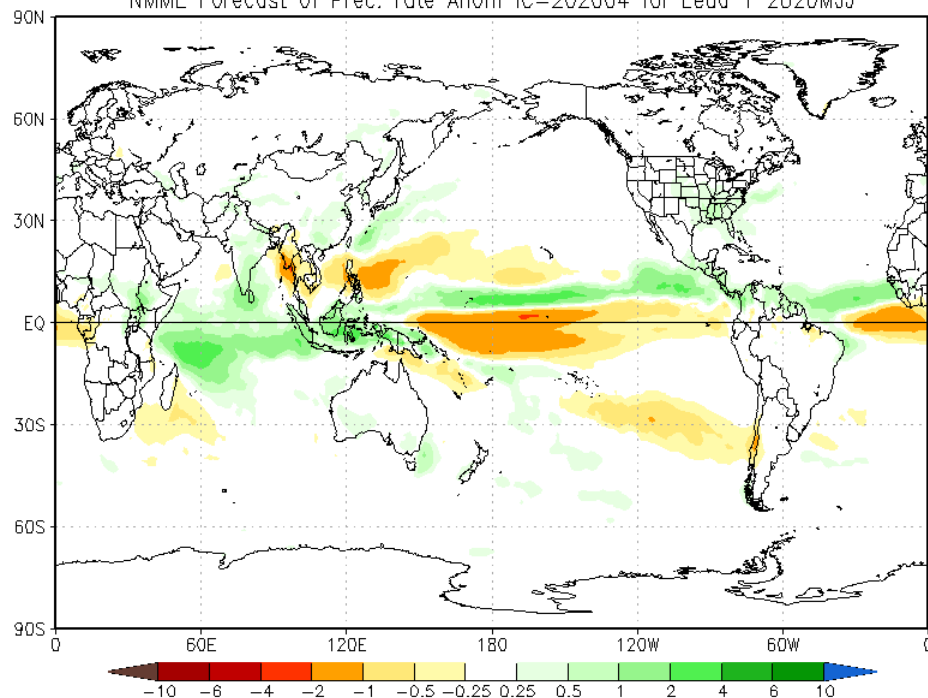
NMME Forecast of Prec. rate Anom IC=202004 for Lead 1 2020MJJ
