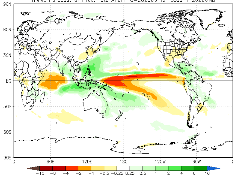
NMME Forecast of Prec. rate Anom IC=202009 for Lead 1 2020OND
