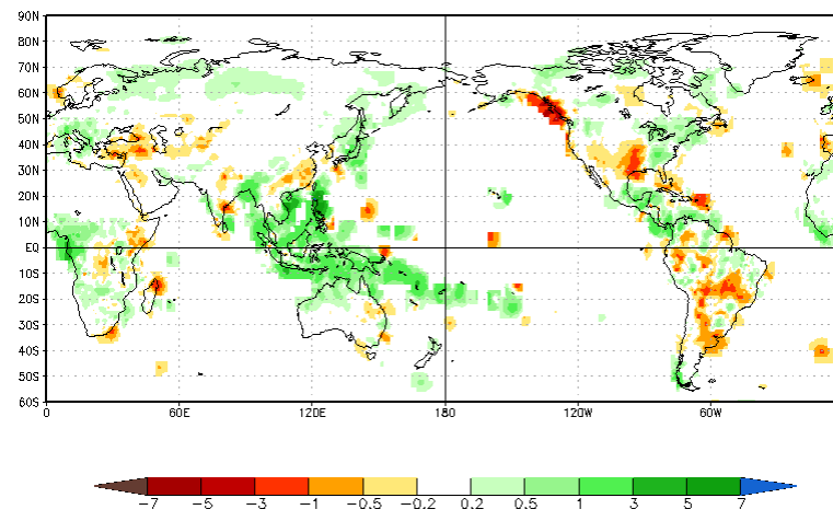
CA Prec Prd for OND2020, ICs through Dec2020(mm/day), Lead -3
