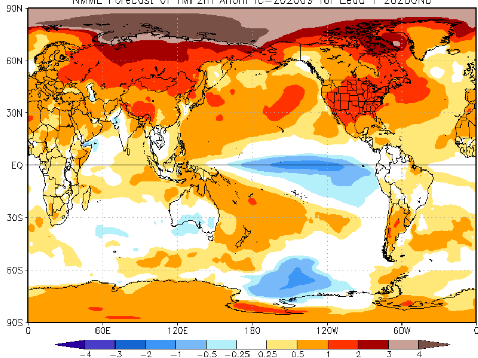
NMME Forecast of TMP2m Anom IC=202009 for Lead 1 2020OND
