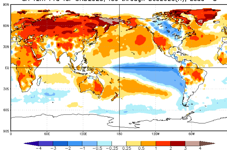
CA T2m Prd for OND2020, ICs through Dec2020(K), Lead -3
