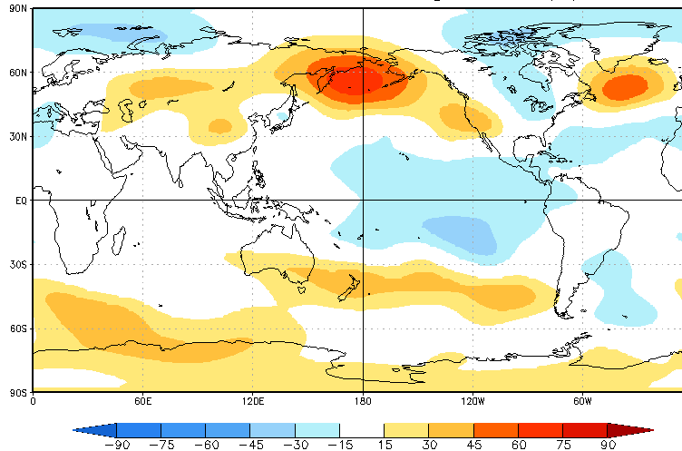
CA HGT200 Prd for OND2020, ICs through Dec2020(m), Lead -3
