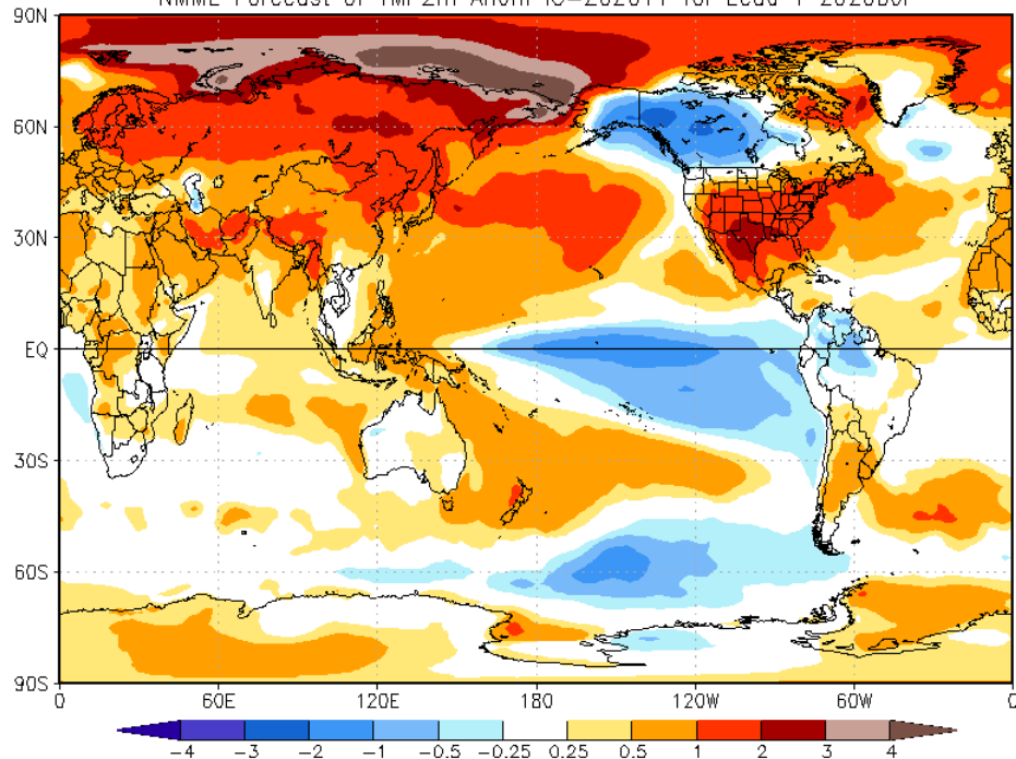
NMME Forecast of TMP2m Anom IC=202011 for Lead 1 2020DJF
