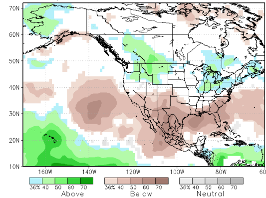
NMME prob fcst Prate IC=202011 for lead 1 2020 DJF
