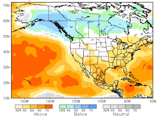
NMME prob fcst TMP2m IC=202011 for lead 1 2020 DJF
