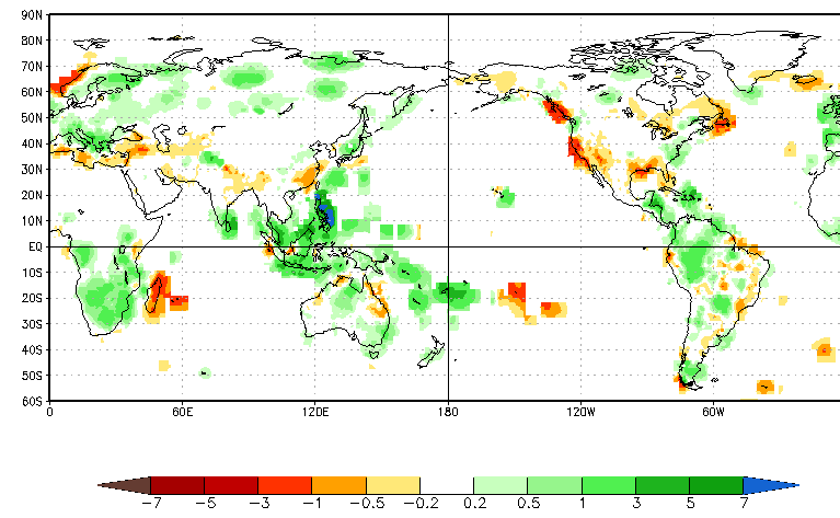
CA Prec Prd for DJF2020/2021, ICs through Feb2021(mm/day), Lead -3
