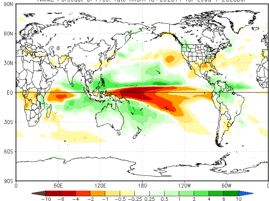
NMME Forecast of Prec. rate Anom IC=202011 for Lead 1 2020DJF
