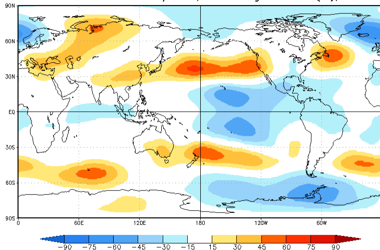
CA HGT200 Prd for DJF2020/2021, ICs through Feb2021(m), Lead -3
