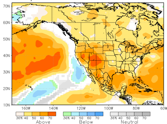
NMME prob fcst TMP2m IC=202104 for lead 1 2021 MJJ
