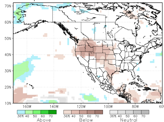
NMME prob fcst Prate IC=202104 for lead 1 2021 MJJ
