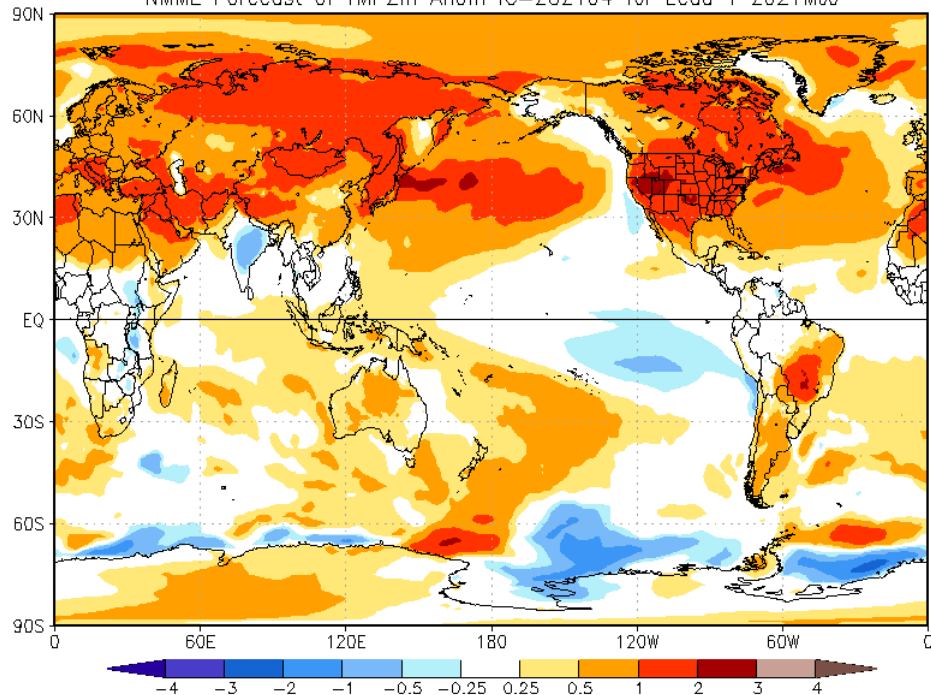
NMME Forecast of TMP2m Anom IC=202104 for Lead 1 2021MJJ
