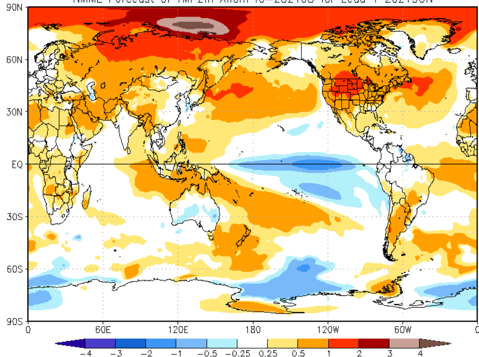
NMME Forecast of TMP2m Anom IC=202108 for Lead 1 2021SON
