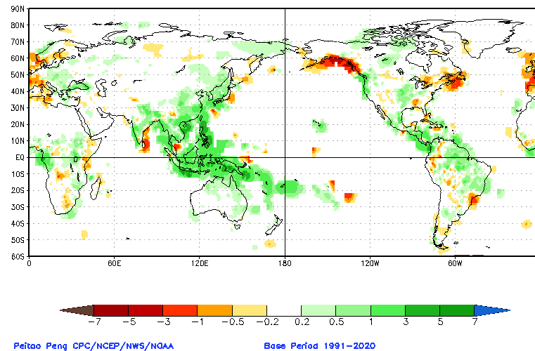
CA Prec Prd for SON2021, ICs through Nov2021(mm/day), Lead -3
