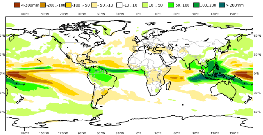
C3S multi-system seasonal forecast ECMWF/Met Office/Météo-France/CMCC/DWD/NCEP/JMA/ECCC Mean precipitation anomaly SON 2021 Nominal forecast start: 01/08/21 Variance-standardized mean
