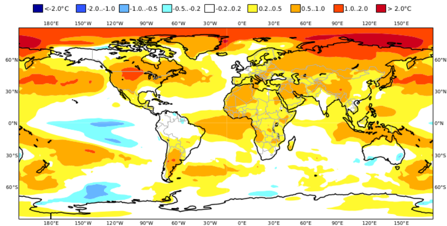
C3S multi-system seasonal forecast ECMWF/Met Office/Météo-France/CMCC/DWD/NCEP/JMA/ECCC Mean 2m temperature anomaly SON 2021 Nominal forecast start: 01/08/21 Variance-standardized mean
