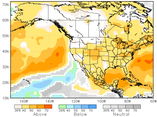
NMME prob fcst TMP2m IC=202108 for lead 1 2021 SON
