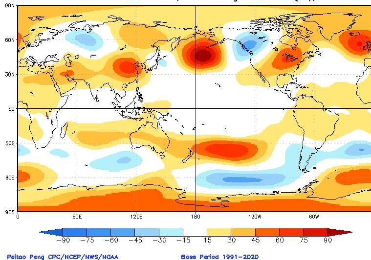
CA HGT200 Prd for SON2021, ICs through Nov2021(m), Lead -3
