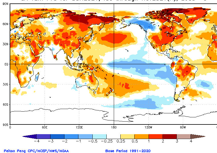
CA T2m Prd for SON2021, ICs through Nov2021(K), Lead -3
