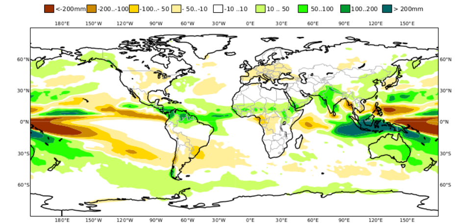
C3S multi-system seasonal forecast ECMWF/Met Office/Météo-France/CMCC/DWD/NCEP/JMA/ECCC Mean precipitation anomaly JAS 2022 Nominal forecast start: 01/06/22 Variance-standardized mean
