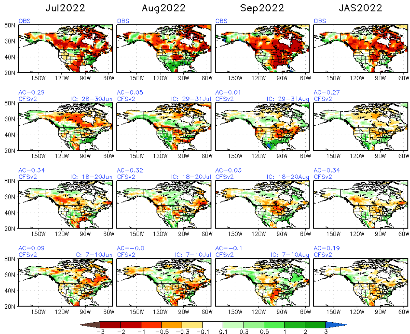
Monthly Means from Monthly Fcst JAS2022 Prec(mm/day) & Obs
