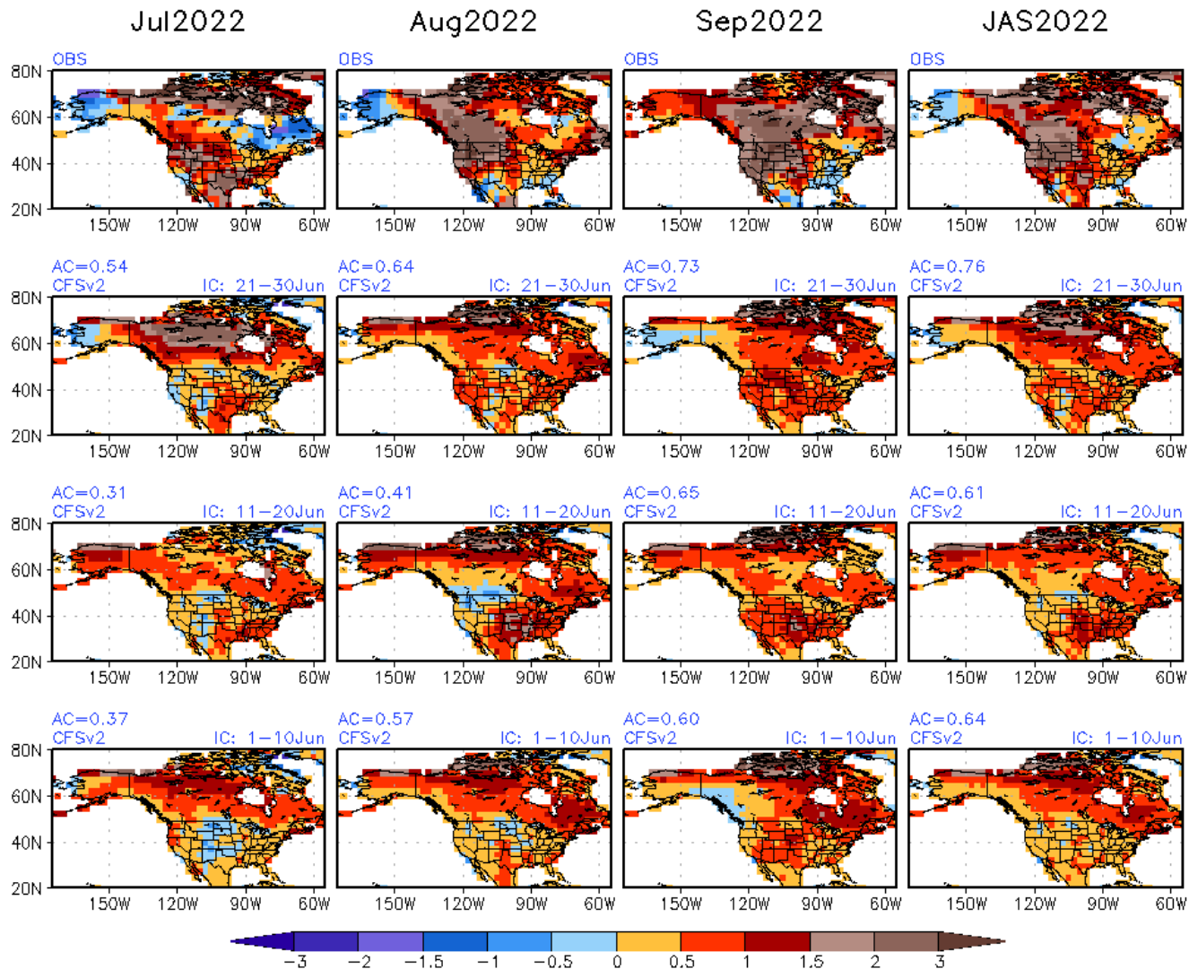
Monthly Means from Seasonal Fcst (40ensm) JAS2022 T2m(K) & Obs
