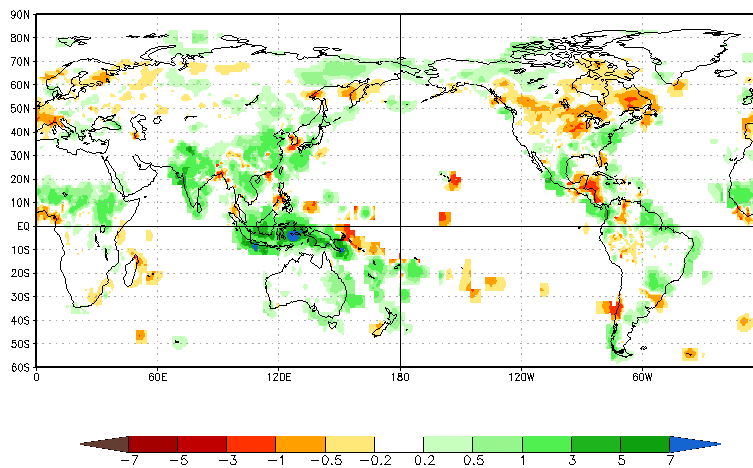
CA Prec Prd for JAS2022, ICs through Sep2022(mm/day), Lead -3
