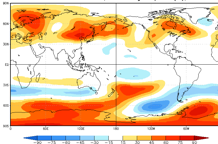
CA HGT200 Prd for JAS2022, ICs through Sep2022(m), Lead -3
