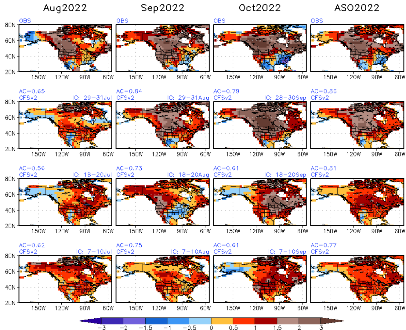
Monthly Means from Monthly Fcst ASO2022 T2m(K) & Obs
