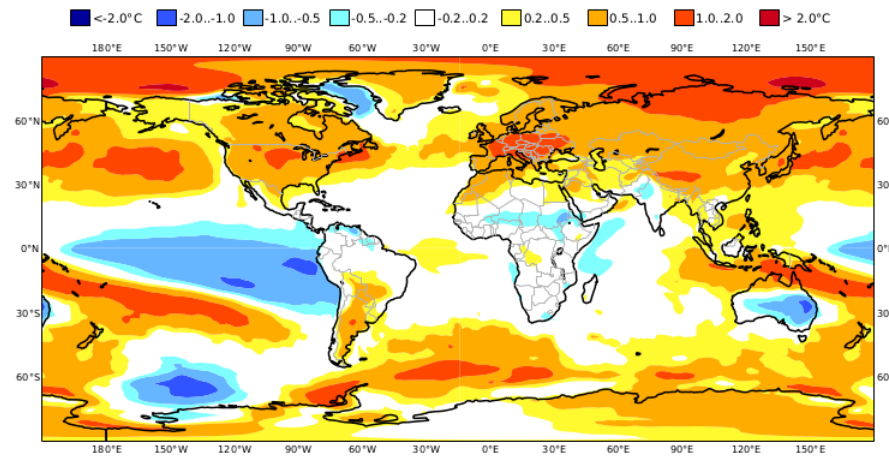
C3S multi-system seasonal forecast ECMWF/Met Office/Météo-France/CMCC/DWD/NCEP/JMA/ECCC Mean 2m temperature anomaly ASO 2022 Nominal forecast start: 01/07/22 Variance-standardized mean
