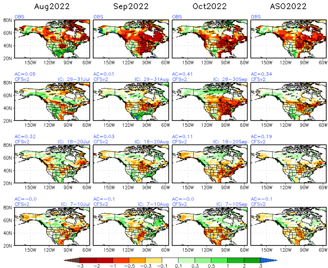
Monthly Means from Monthly Fcst ASO2022 Prec(mm/day) & Obs
