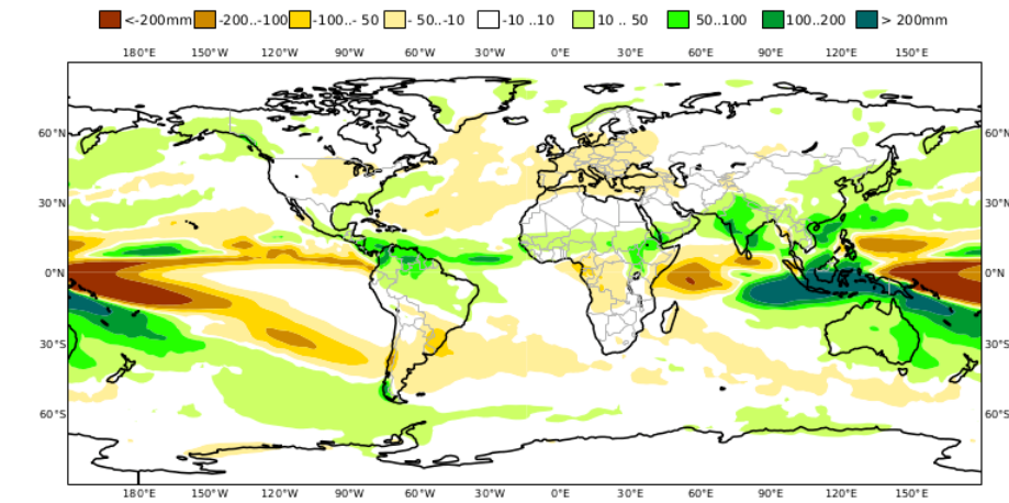
C3S multi-system seasonal forecast ECMWF/Met Office/Météo-France/CMCC/DWD/NCEP/JMA/ECCC Mean precipitation anomaly ASO 2022 Nominal forecast start: 01/07/22 Variance-standardized mean
