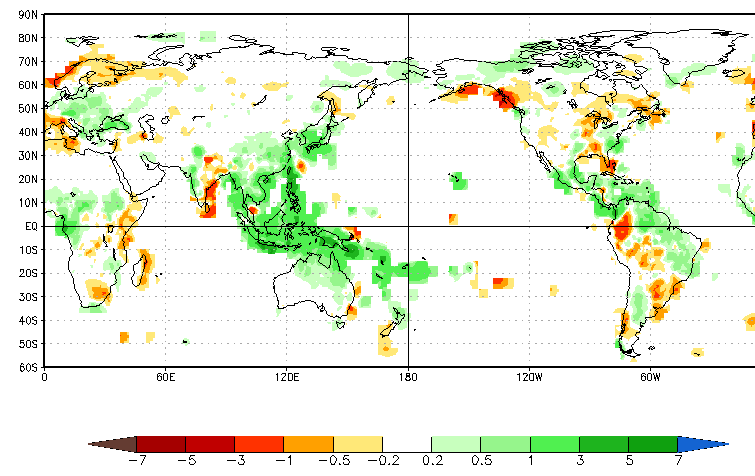
CA Prec Prd for SON2022, ICs through Nov2022(mm/day), Lead -3
