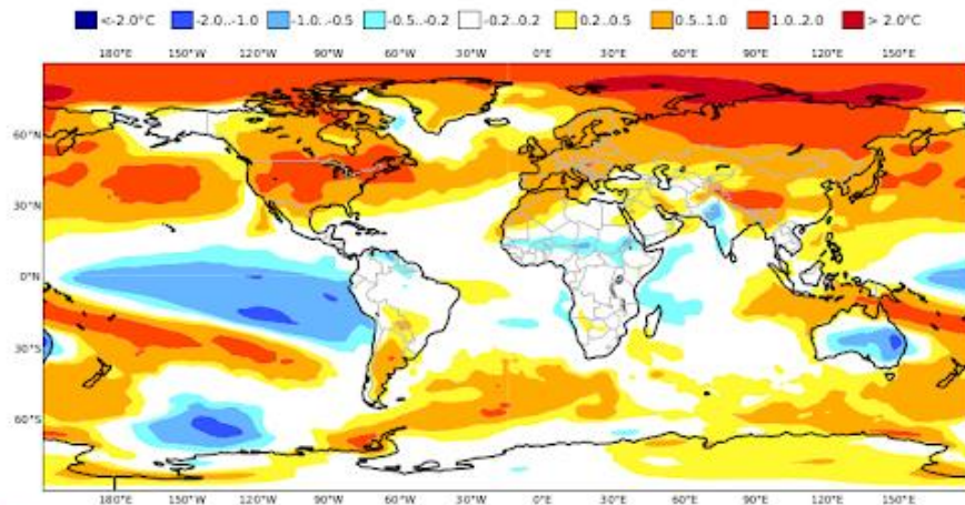
C3S multi-system seasonal forecast ECMWF/Met Office/Météo-France/CMCC/DWD/NCEP/JMA/ECCC Mean 2m temperature anomaly Nominal forecast start: 01/08/22 Variance-standardized mean SON 2022
