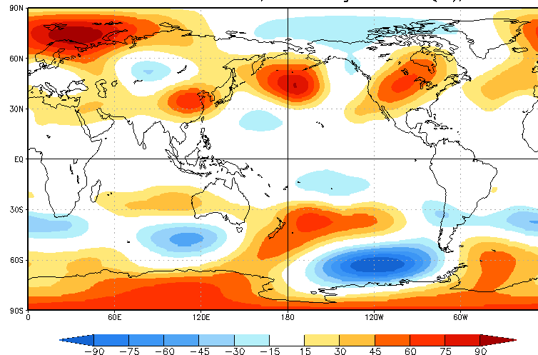
CA HGT200 Prd for SON2022, ICs through Nov2022(m), Lead -3
