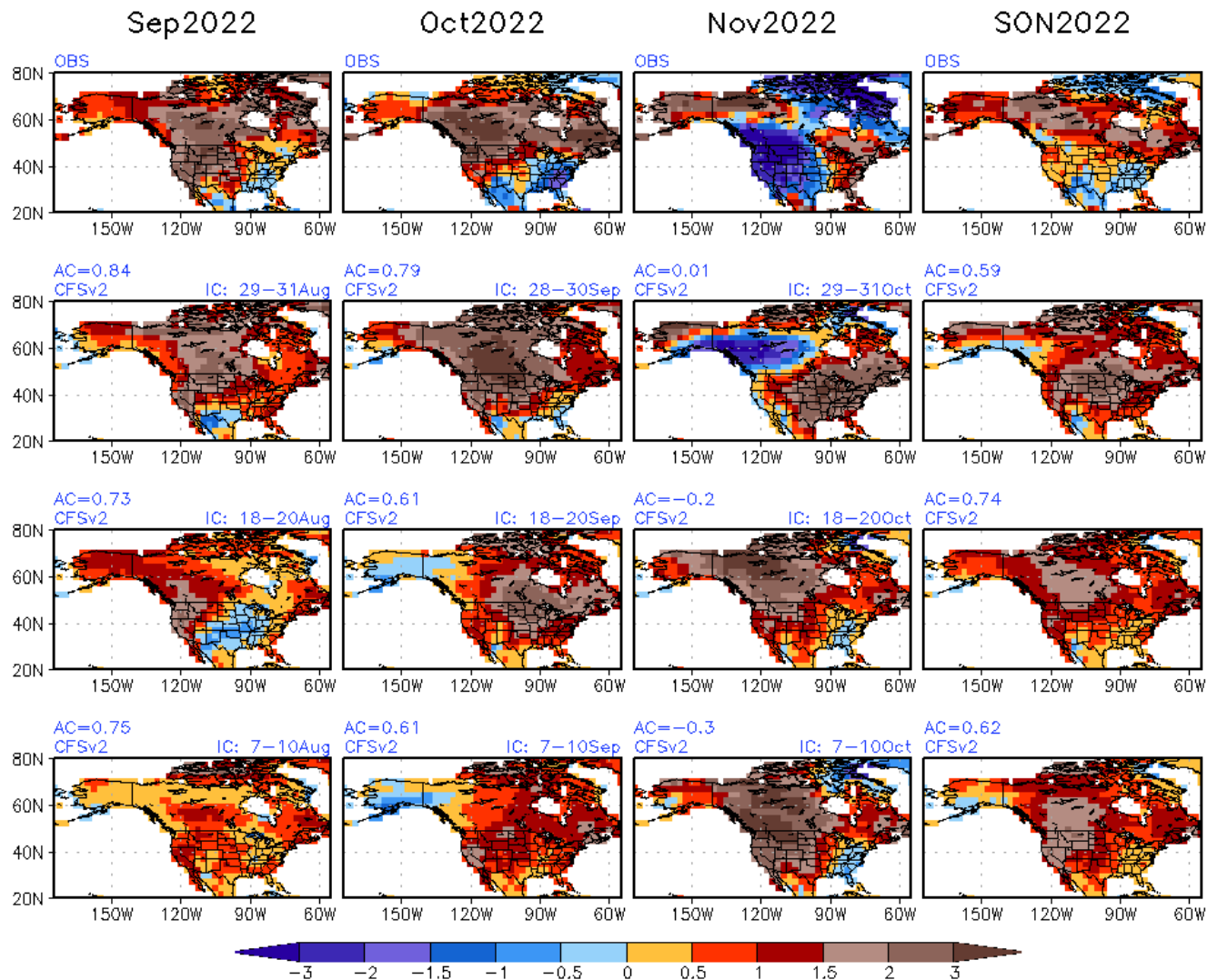
Monthly Means from Monthly Fcst SON2022 T2m(K) & Obs
