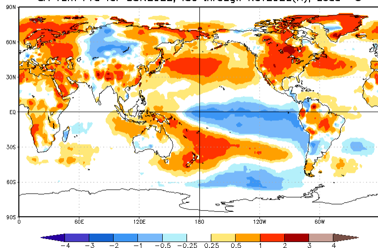
CA T2m Prd for SON2022, ICs through Nov2022(K), Lead -3
