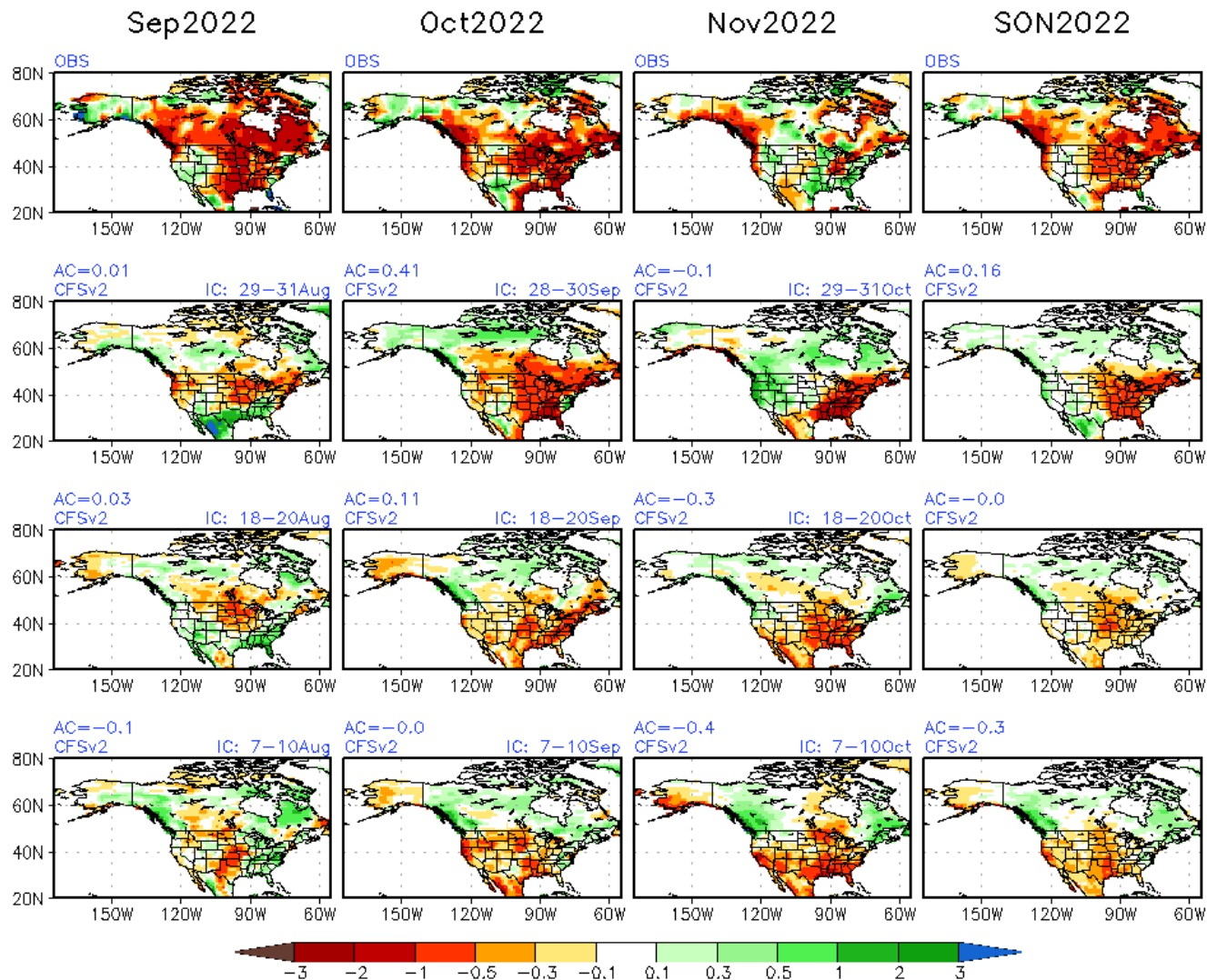
Monthly Means from Monthly Fcst SON2022 Prec(mm/day) & Obs
