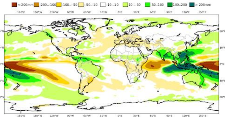
C3S multi-system seasonal forecast ECMWF/Met Office/Météo-France/CMCC/DWD/NCEP/JMA/ECCC Mean precipitation anomaly Nominal forecast start: 01/08/22 Variance-standardized mean SON 2022
