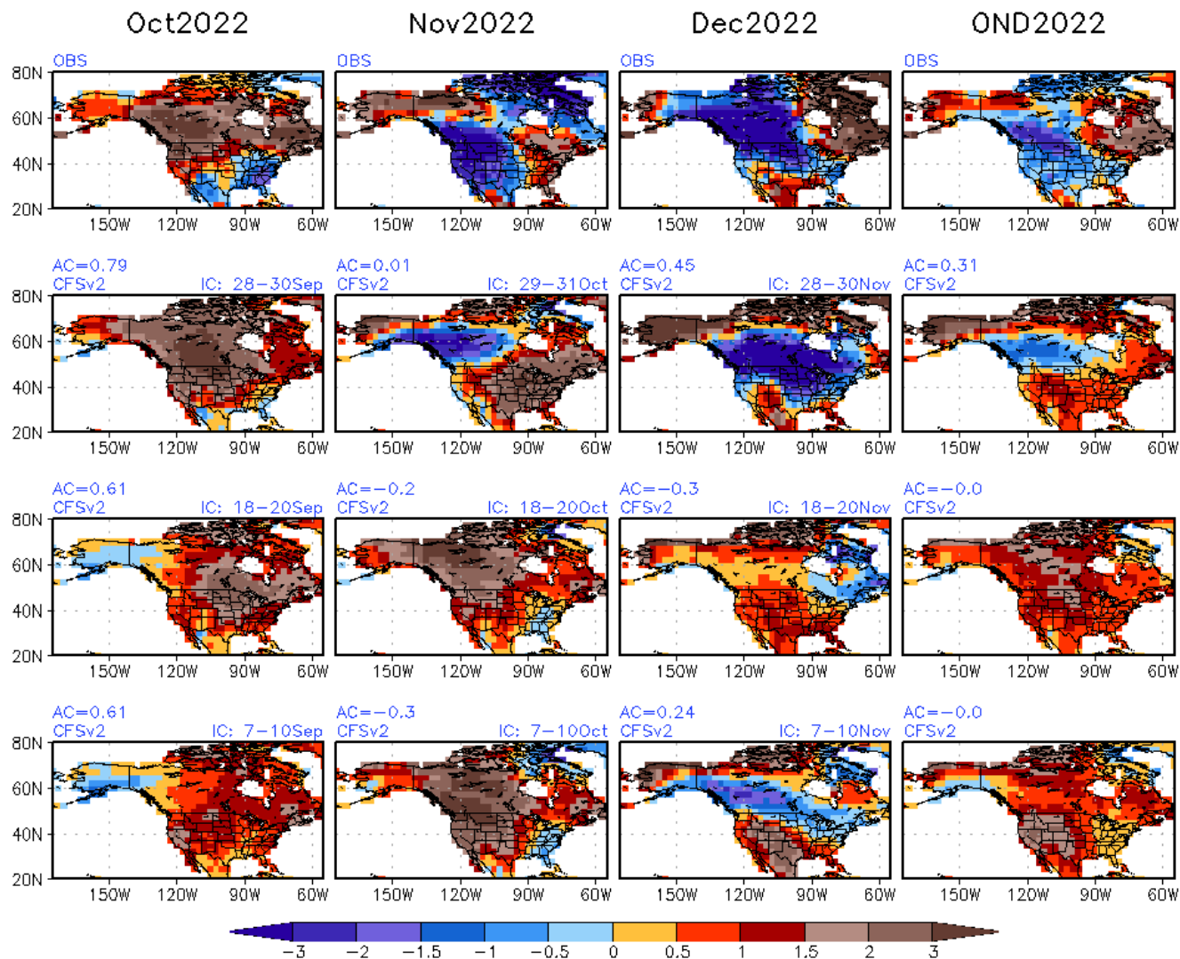
Monthly Means from Monthly Fcst OND2022 T2m(K) & Obs
