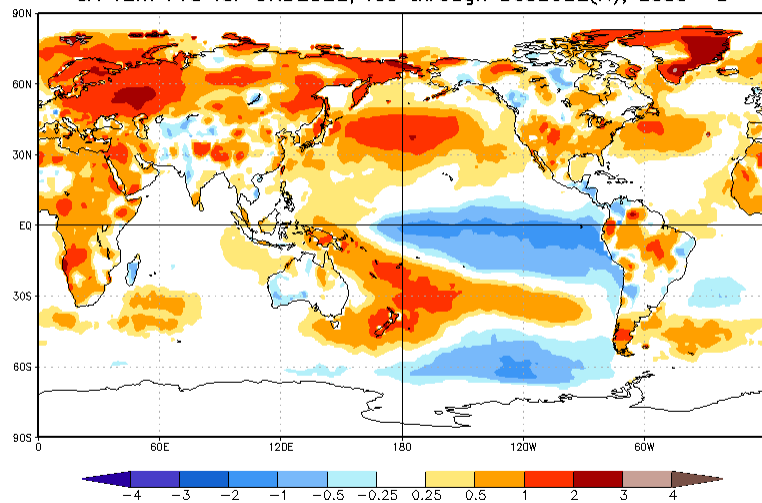
CA T2m Prd for OND2022, ICs through Dec2022(K), Lead -3
