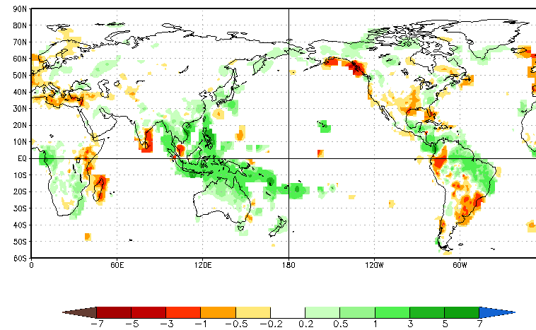
CA Prec Prd for OND2022, ICs through Dec2022(mm/day), Lead -3
