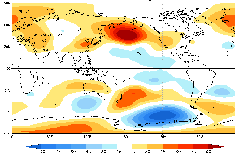
CA HGT200 Prd for OND2022, ICs through Dec2022(m), Lead -3
