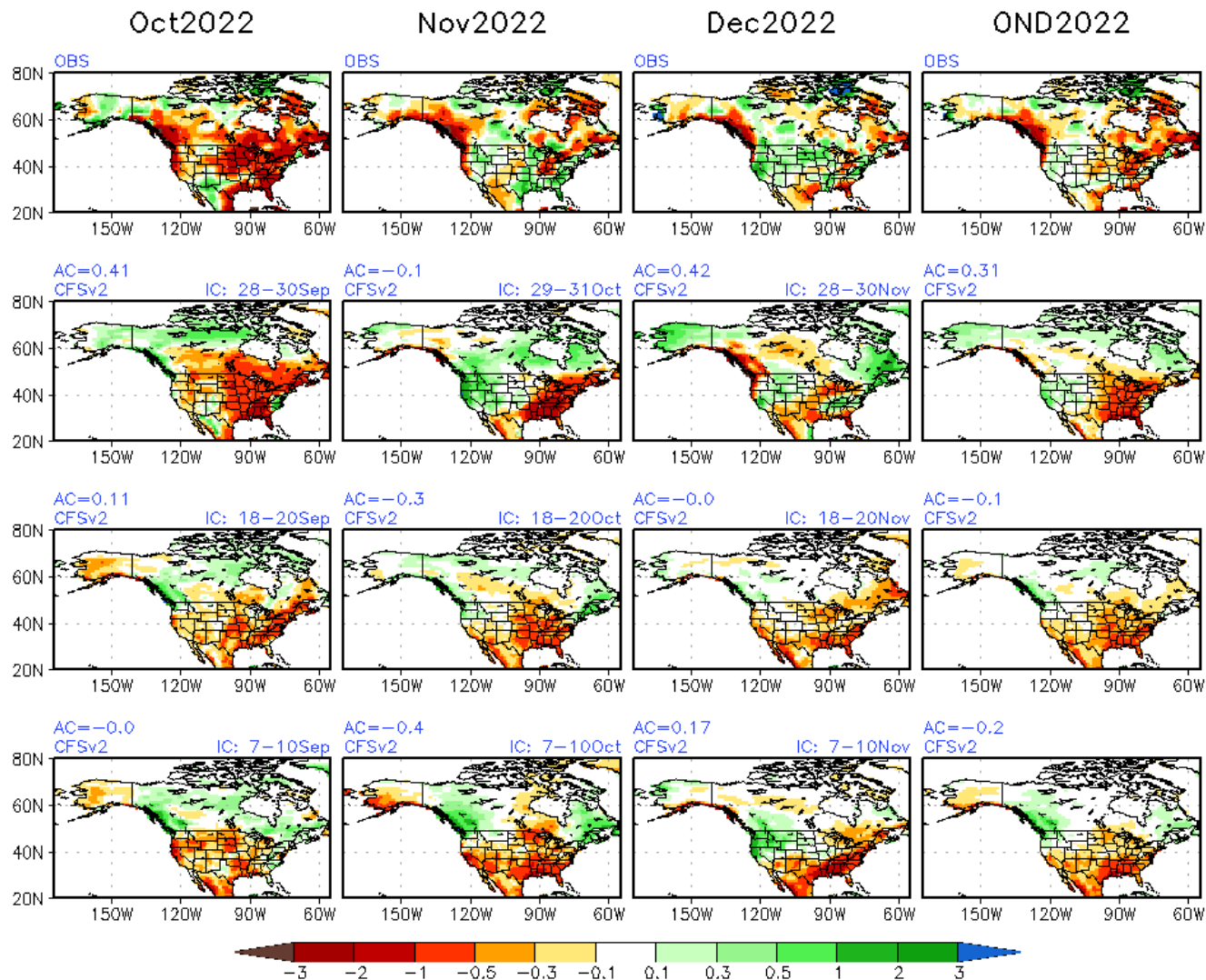
Monthly Means from Monthly Fcst OND2022 Prec(mm/day) & Obs
