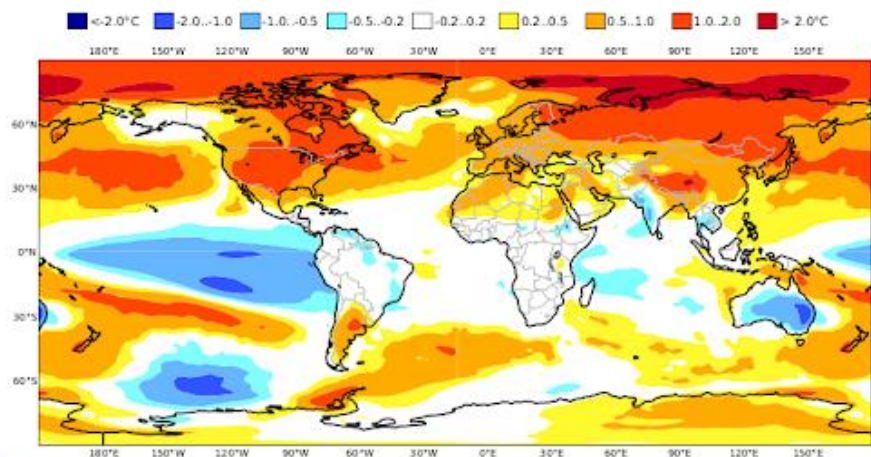
C3S multi-system seasonal forecast Mean 2m temperature anomaly Nominal forecast start: 01/09/22 Variance-standardized mean ECMWF/Met Office/Météo-France/CMCC/DWD/NCEP/JMA/ECCC OND 2022
