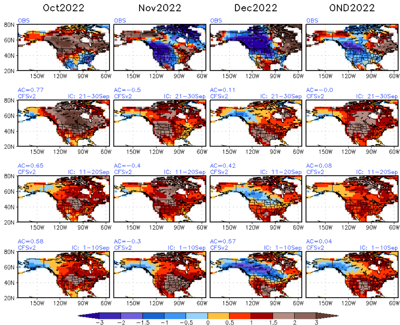
Monthly Means from Seasonal Fcst (40ensm) OND2022 T2m(K) & Obs
