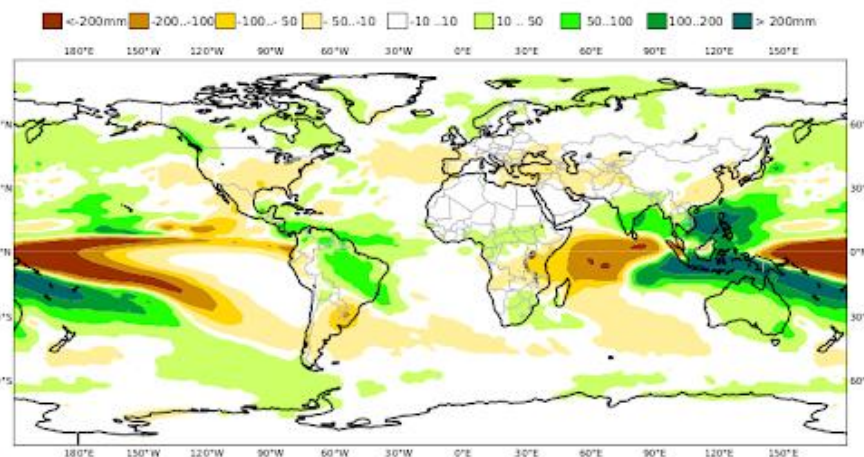
C3S multi-system seasonal forecast Mean precipitation anomaly Nominal forecast start: 01/09/22 Variance-standardized mean ECMWF/Met Office/Météo-France/CMCC/DWD/NCEP/JMA/ECCC OND 2022
