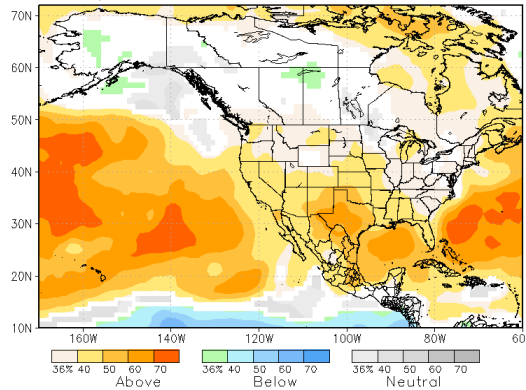
NMME prob fcast TMP2m IC=202210 for lead 1 2022 NDJ
