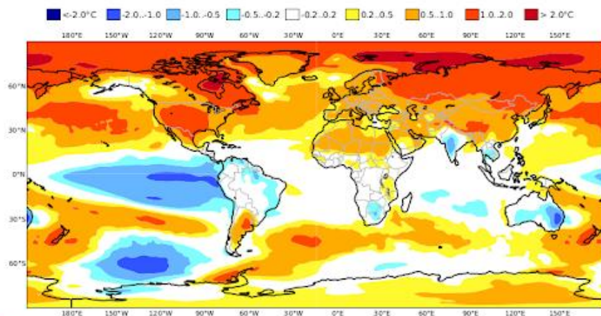
C3S multi-system seasonal forecast Mean 2m temperature anomaly Nominal forecast start: 01/10/22 Variance-standardized mean ECMWF/Met Office/Météo-France/CMCC/DWD/NCEP/JMA/ECCC NDJ 2022/23
