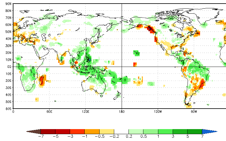
CA Prec Prd for NDJ2022/2023, ICs through Jan2023(mm/day), Lead -3
