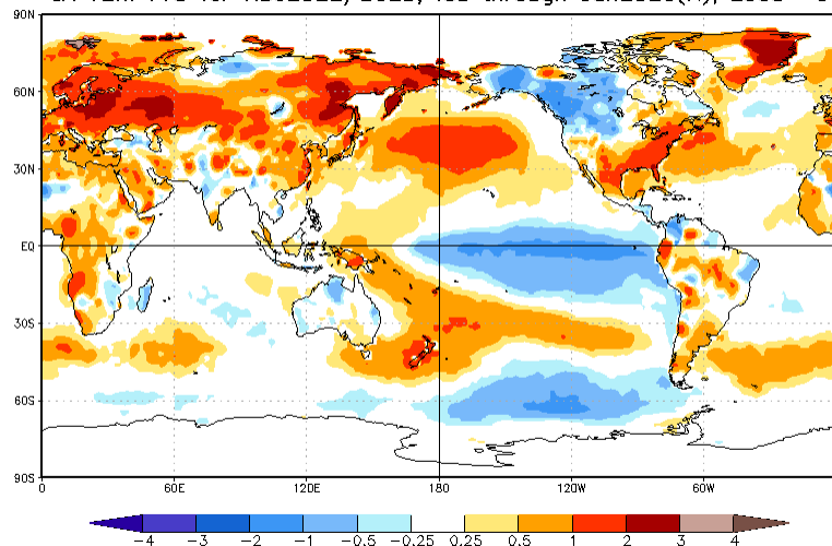
CA T2m Prd for NDJ2022/2023, ICs through Jan2023(K), Lead -3
