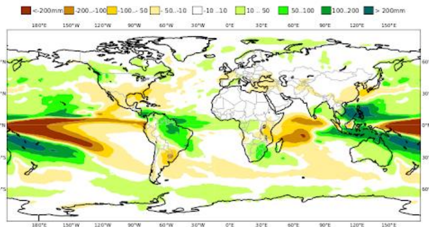
C3S multi-system seasonal forecast Mean precipitation anomaly Nominal forecast start: 01/10/22 Variance-standardized mean ECMWF/Met Office/Météo-France/CMCC/DWD/NCEP/JMA/ECCC NDJ 2022/23
