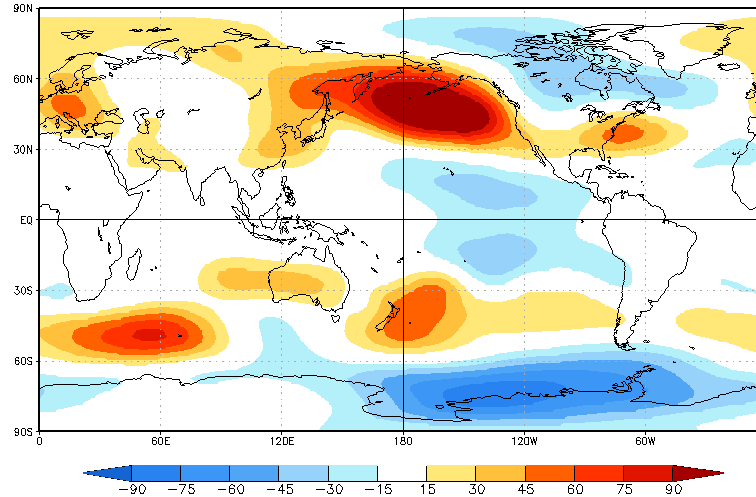
CA HGT200 Prd for NDJ2022/2023, ICs through Jan2023(m), Lead -3
