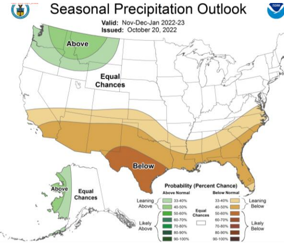
NMME prob fcast Prate IC=202210 for lead 1 2022 NDJ
