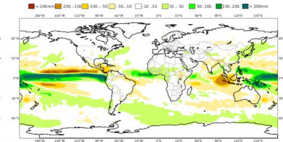
C3S multi-system seasonal forecast Mean precipitation anomaly Nominal forecast start: 01/04/23 Variance-standardized mean ECMWF/Met Office/Météo-France/CMCC/DWD/NCEP/JMA/ECCC MJJ 2023
