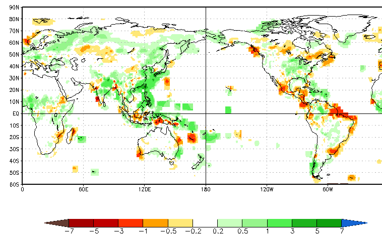
CA Prec Prd for MJJ2023, ICs through Jul2023(mm/day), Lead -3
