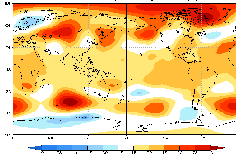
CA HGT200 Prd for MJJ2023, ICs through Jul2023(m), Lead -3
