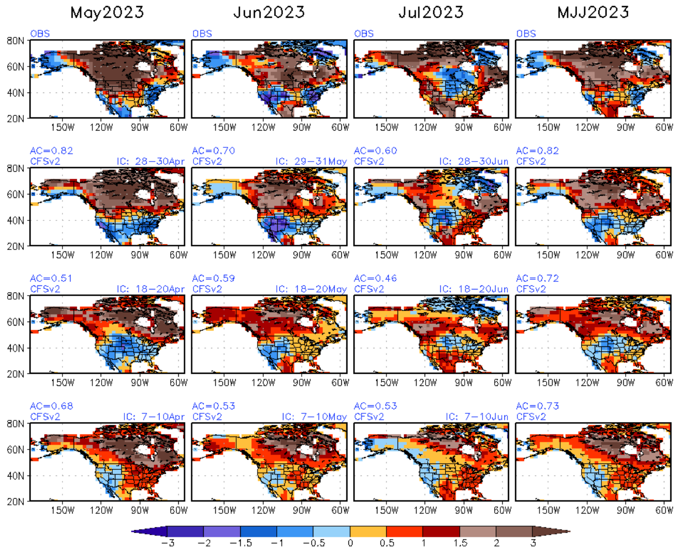
Monthly Means from Monthly Fcst MJJ2023 T2m(K) & Obs
