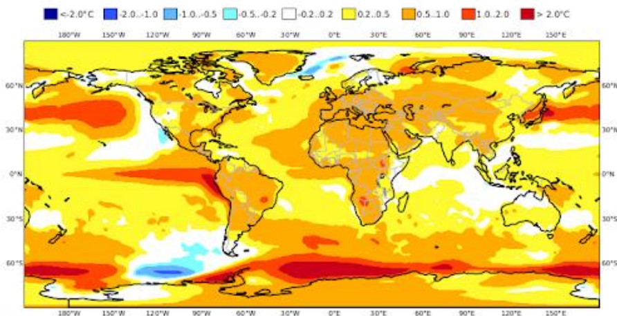
C3S multi-system seasonal forecast Mean 2m temperature anomaly Nominal forecast start: 01/04/23 Variance-standardized mean ECMWF/Met Office/Météo-France/CMCC/DWD/NCEP/JMA/ECCC MJJ 2023
