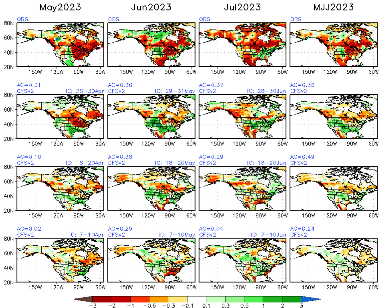
Monthly Means from Monthly Fcst MJJ2023 Prec(mm/day) & Obs
