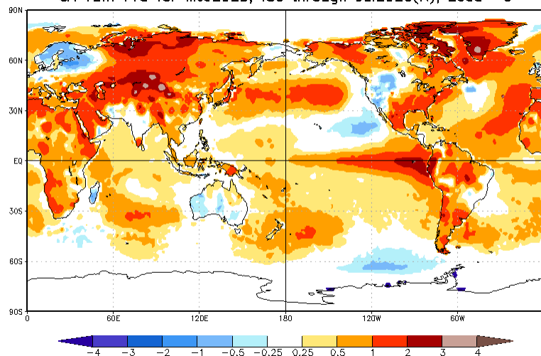
CA T2m Prd for MJJ2023, ICs through Jul2023(K), Lead -3
