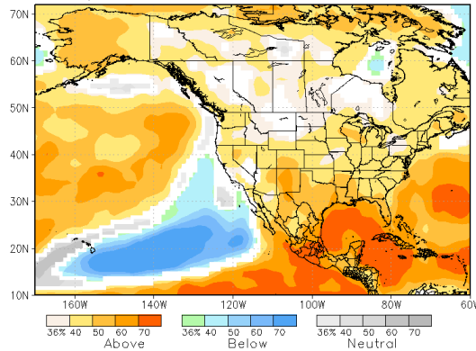
NMME prob fcst TMP2m IC=202307 for lead 1 2023 ASO
