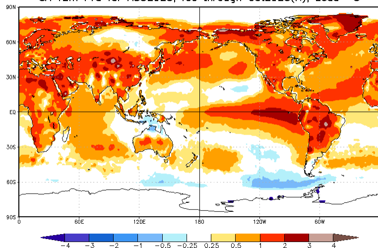
CA T2m Prd for ASO2023, ICs through Oct2023(K), Lead -3
