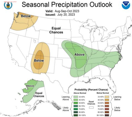
NMME prob fcst Prate IC=202307 for lead 1 2023 ASO
