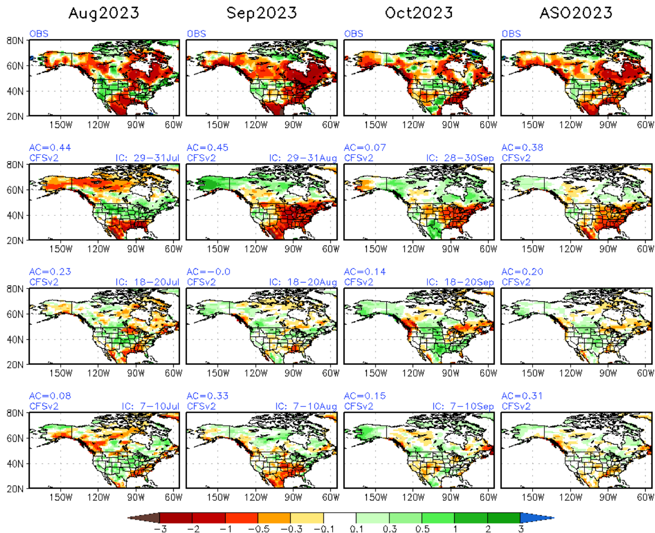
Monthly Means from Monthly Fcst ASO2023 Prec(mm/day) & Obs
