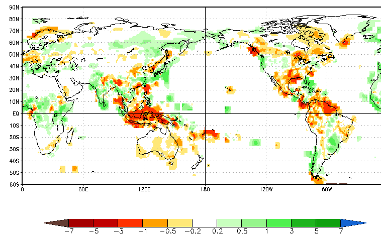
CA Prec Prd for ASO2023, ICs through Oct2023(mm/day), Lead -3
