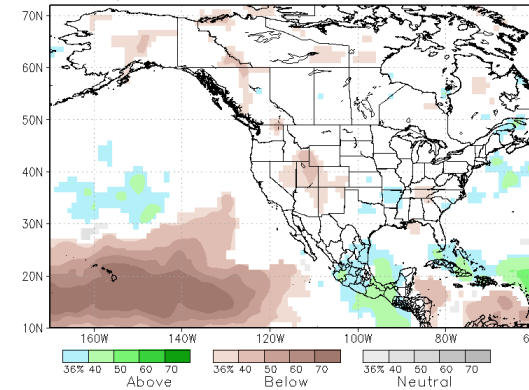
NMME prob fcst Prate IC=202307 for lead 1 2023 ASO
