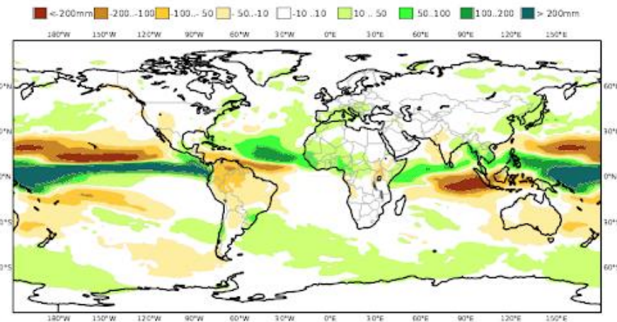
C3S multi-system seasonal forecast Mean precipitation anomaly Nominal forecast start: 01/07/23 Variance-standardized mean ECMWF/Met Office/Météo-France/CMCC/DWD/NCEP/JMA/ECCC ASO 2023
