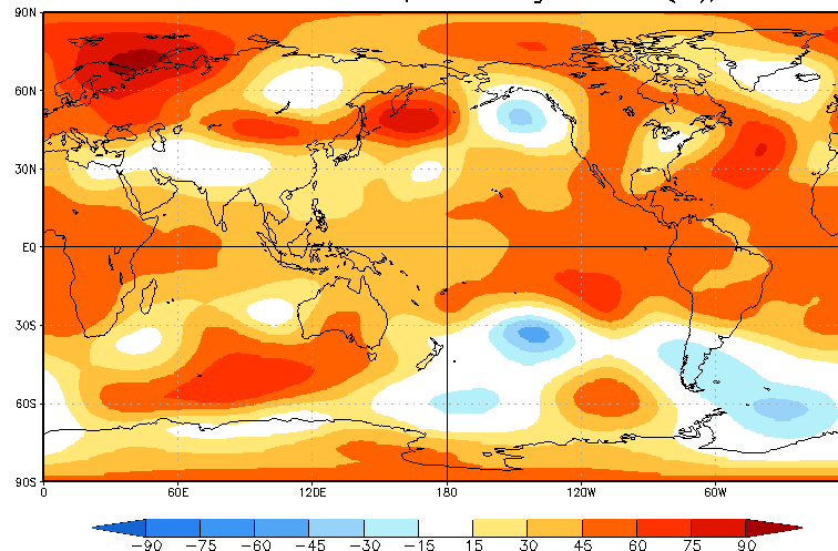
CA HGT200 Prd for ASO2023, ICs through Oct2023(m), Lead -3
