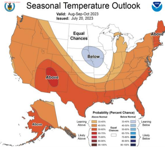
NMME prob fcst TMP2m IC=202307 for lead 1 2023 ASO
