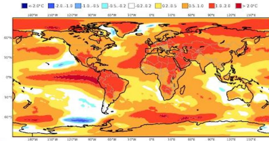
C3S multi-system seasonal forecast Mean 2m temperature anomaly Nominal forecast start: 01/07/23 Variance-standardized mean ECMWF/Met Office/Météo-France/CMCC/DWD/NCEP/JMA/ECCC ASO 2023
