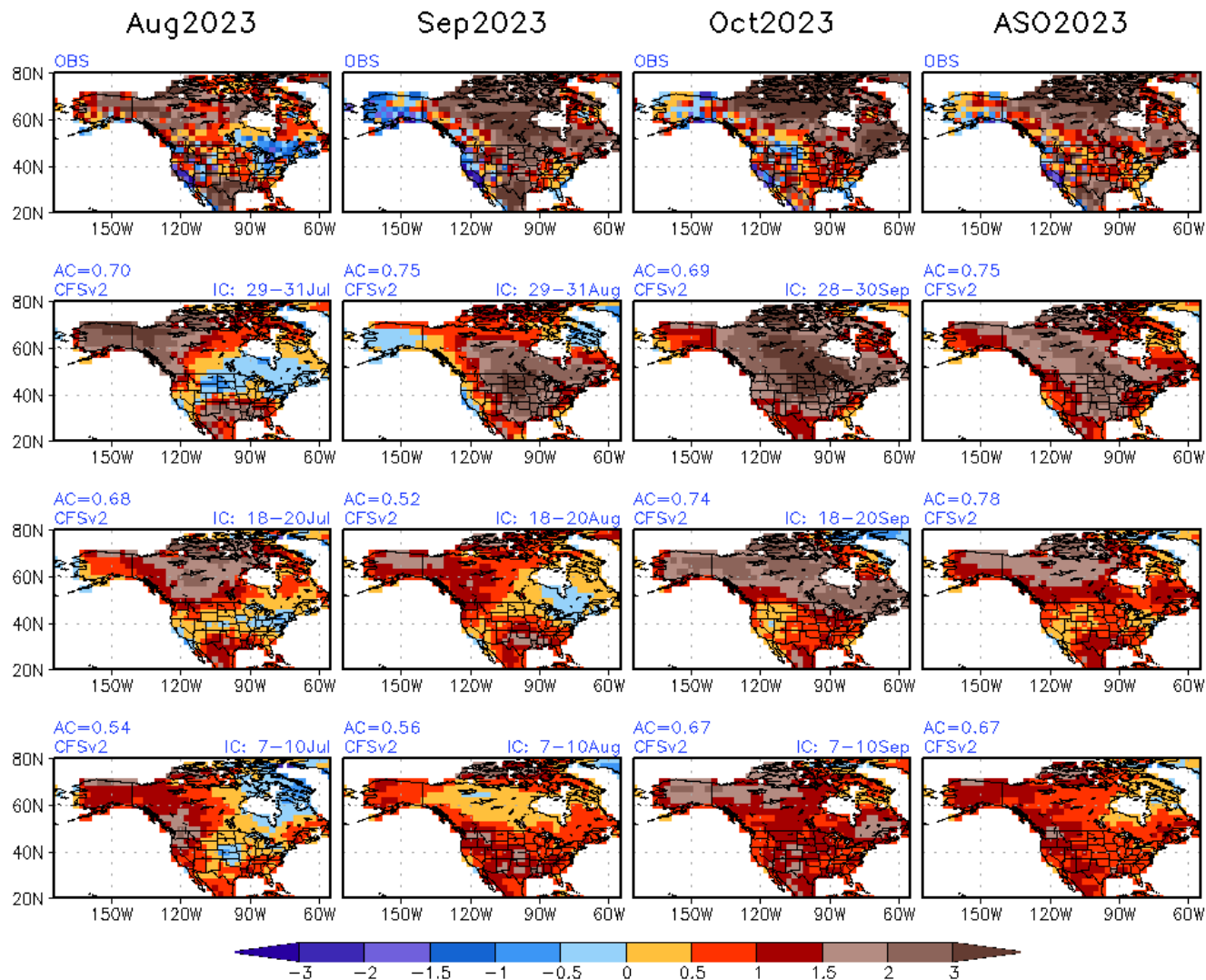
Monthly Means from Monthly Fcst ASO2023 T2m(K) & Obs
