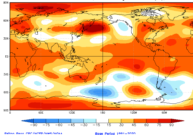
CA HGT200 Prd for SON2023, ICs through Nov2023(m), Lead -3
