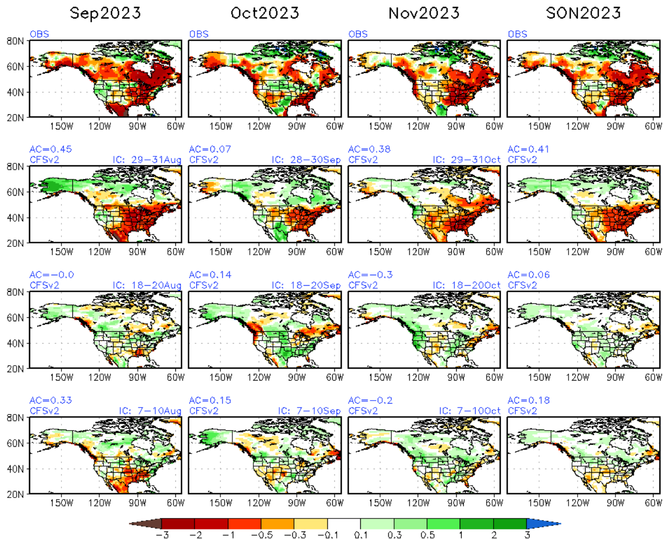
Monthly Means from Monthly Fcst SON2023 Prec(mm/day) & Obs
