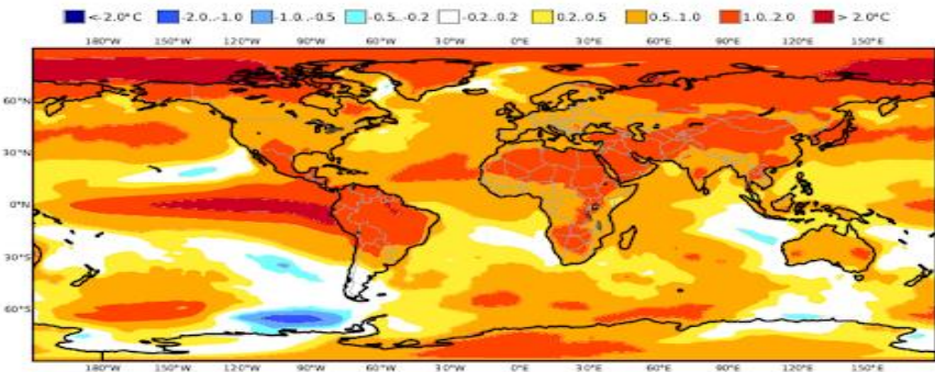
C3S multi-system seasonal forecast ECMWF/Met Office/Météo-France/CMCC/DWD/NCEP/JMA/ECCC Mean 2m temperature anomaly SON 2023 Nominal forecast start: 01/08/23 Variance-standardized mean
