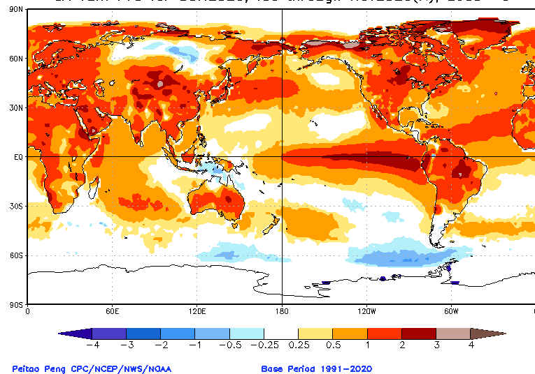
CA T2m Prd for SON2023, ICs through Nov2023(K), Lead -3
