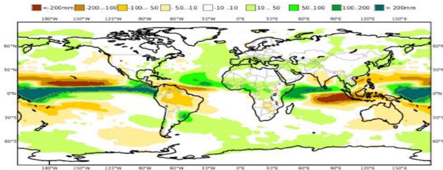
C3S multi-system seasonal forecast ECMWF/Met Office/Météo-France/CMCC/DWD/NCEP/JMA/ECCC Mean precipitation anomaly SON 2023 Nominal forecast start: 01/08/23 Variance-standardized mean
