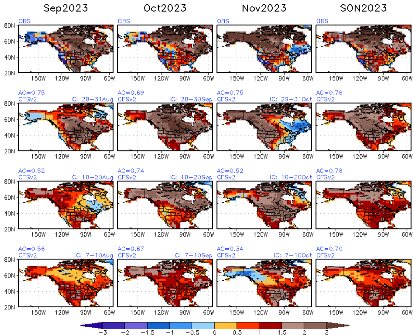
Monthly Means from Monthly Fcst SON2023 T2m(K) & Obs
