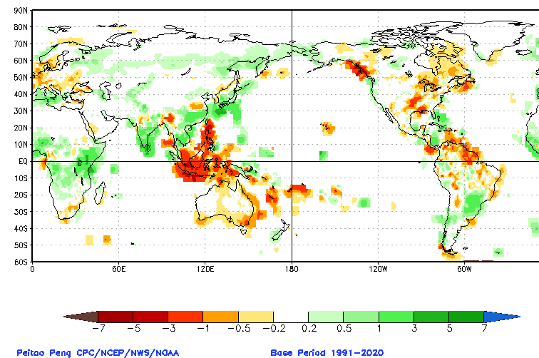
CA Prec Prd for SON2023, ICs through Nov2023(mm/day), Lead -3
