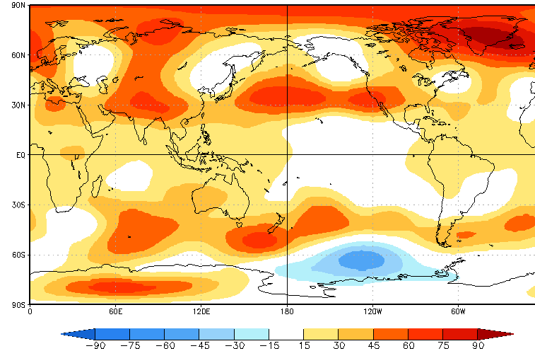
CA HGT200 Prd for FMA2025, ICs through Apr2025(m), Lead -3
