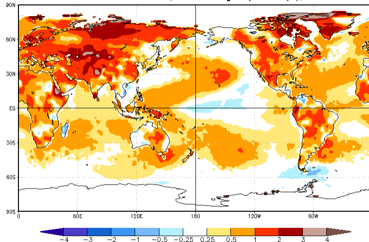
CA T2m Prd for FMA2025, ICs through Apr2025(K), Lead -3
