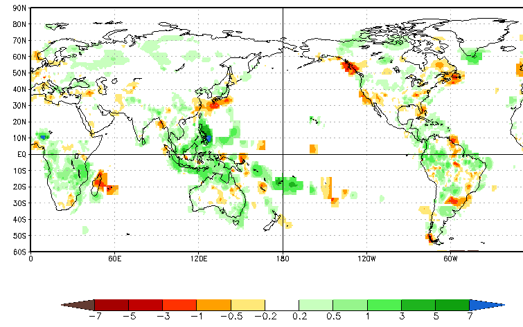
CA Prec Prd for FMA2025, ICs through Apr2025(mm/day), Lead -3
