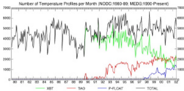
Figure 1. Number of temperature profiles during 1980-2001.
