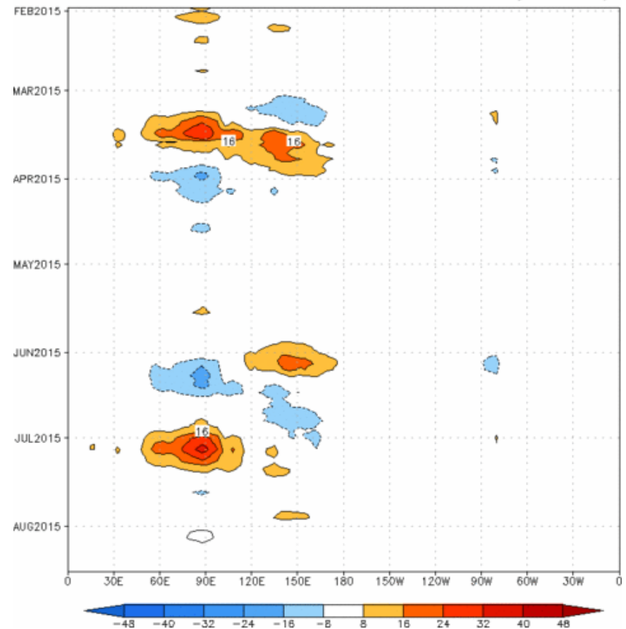
Reconstructed anomaly field associated with the MJO using RMM1 & RMM2 OLR [7.5°S,7.5°N] (cont:4Wm -2 ) Period:31-Jan-2015 to 02-Aug-2015 The unfilled contours are GEFS forecast reconstructed anomaly for 15 days
