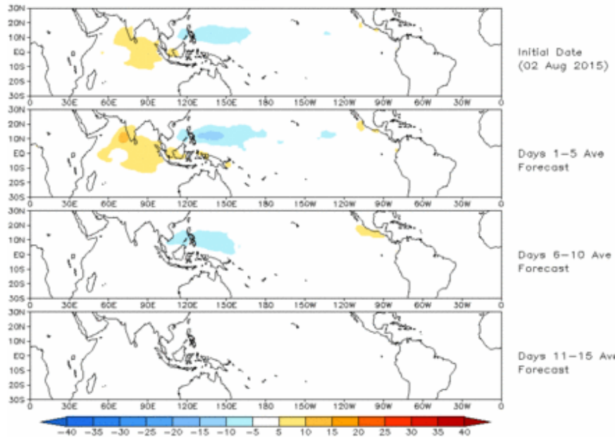
Prediction of MJO-related anomalies using GEFS operational forecast Initial date: 02 Aug 2015 OLR
