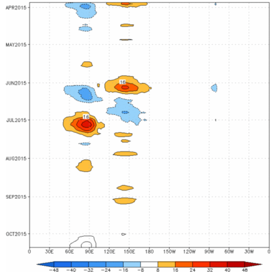
Reconstructed anomaly field associated with the MJO using RMM1 & RMM2 OLR [ 7.5^{\circ} S, 7.5^{\circ} N] (cont: 4\text{Wm}^{-2} ) Period: 28-Mar-2015 to 27-Sep-2015 The unfilled contours are GEFS forecast reconstructed anomaly for 15 days
