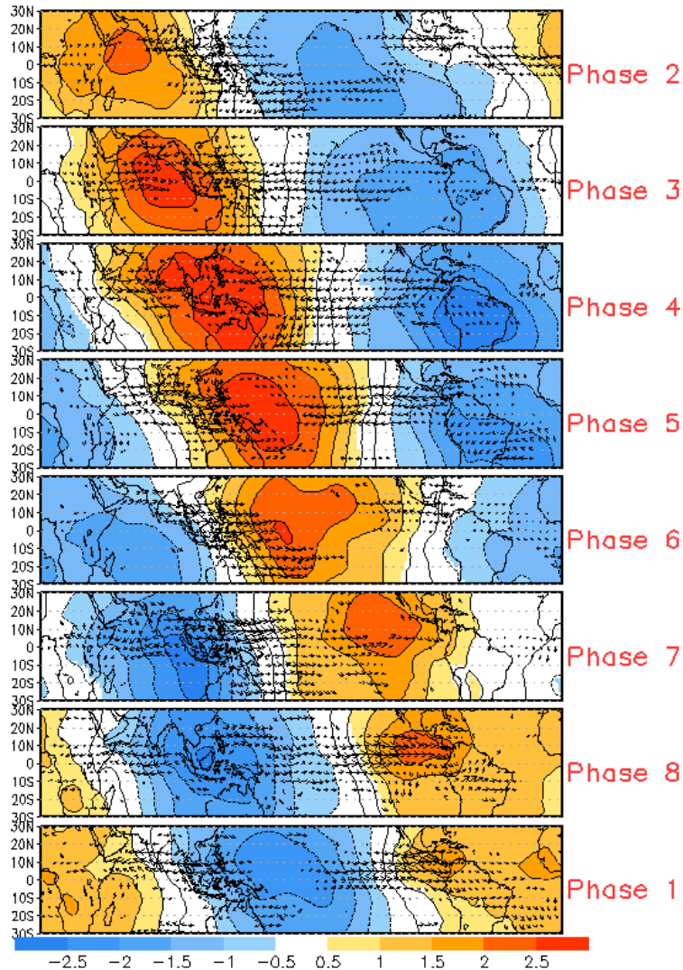
850-hPa Velocity Potential and Wind Anomalies (May - Sep)
